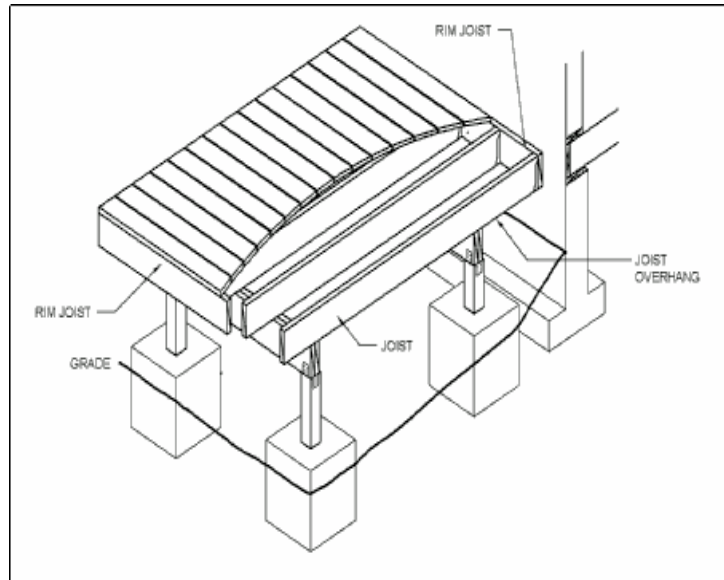
Figure 13 - Free-Standing Deck
