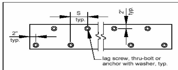
Figure 11 - Ledger Board Fastener Spacing and Clearances
