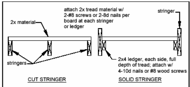
Figure 30 – Tread Connection Requirements
