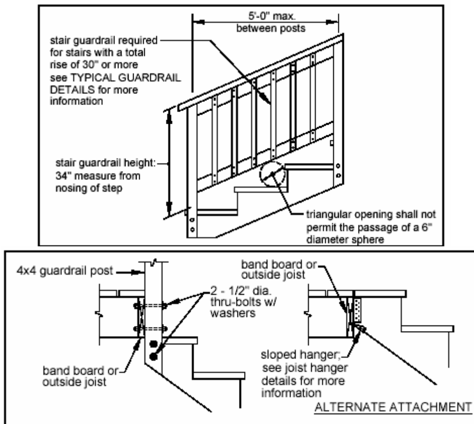
Figure 32 – Stair Stringer Connection Detail
