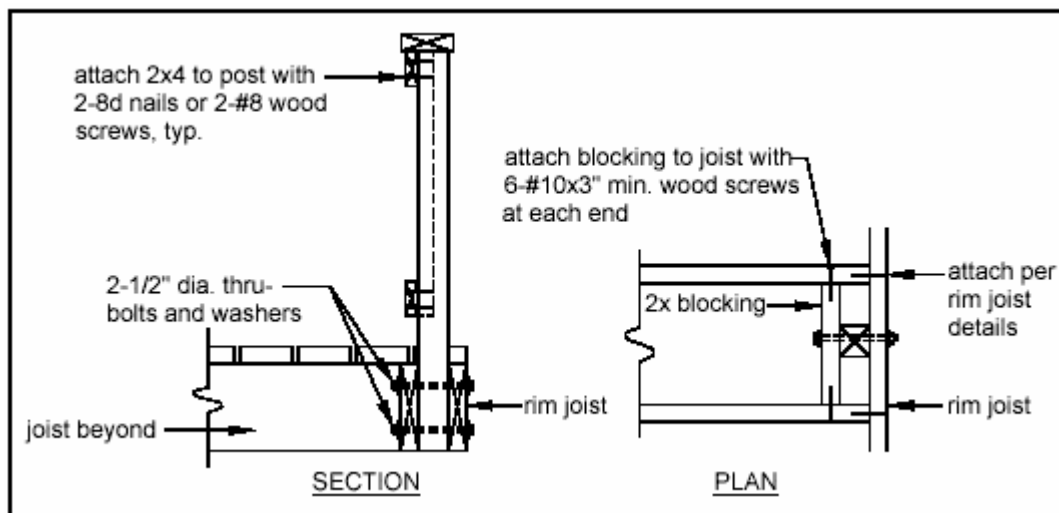
Figure 26 - Guardrail Post to Rim Joist Detail, Option I
