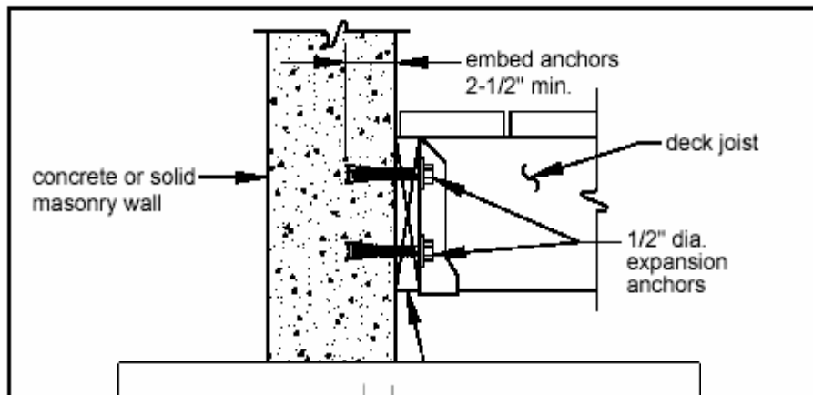
Figure 6 - Attachment of Ledger Board to Concrete or Solid Masonry Wall
