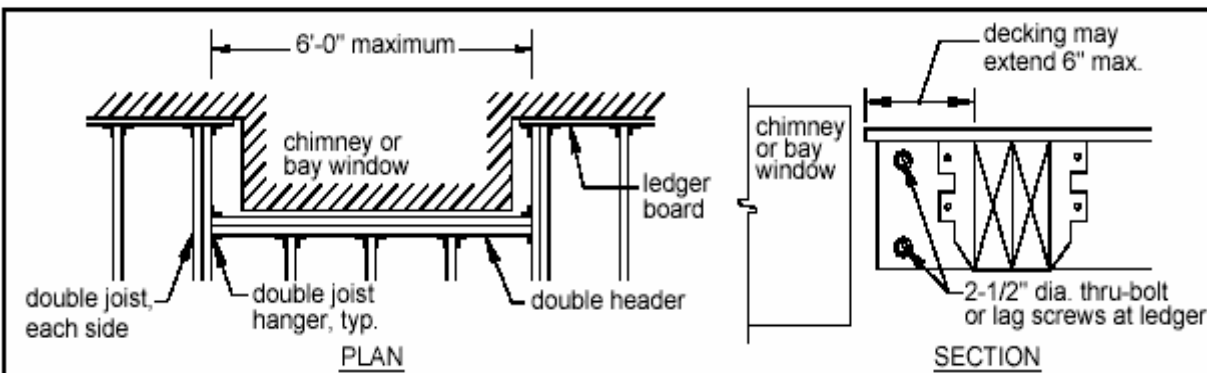
Figure 35 - Requirements for Framing at Chimney or Bay Window
