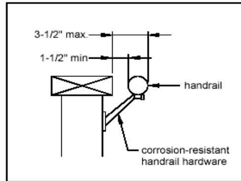
Figure 33 – Handrail Requirements
